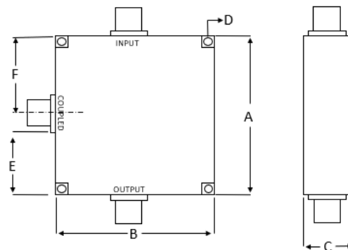
OUTLINE DIMENSIONS (inch/mm)
