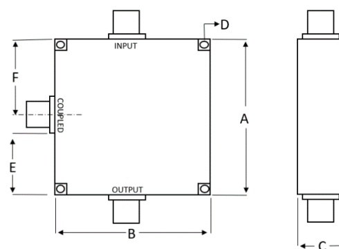
OUTLINE DIMENSIONS (inch/mm)
